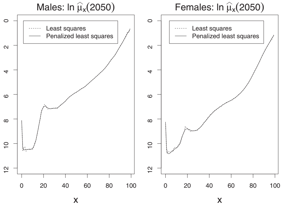
Figure 9 Forces of mortality for the French population in 2050 according to the smoothed Lee–Carter model for mortality projection (males are on the left, females are on the right)
