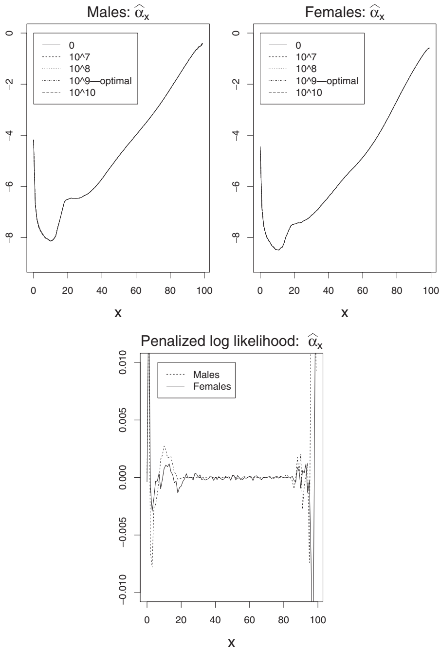
Figure 5 Estimation of the \alpha_x parameters via penalized maximum likelihood for different values of \pi_\beta including the optimal \hat{\pi}_\beta selected by cross validation: estimated \alpha_x 's for males (top left), estimated \alpha_x 's for females (top right) and relative differences between the estimated \alpha_x 's obtained without smoothing ( \pi_\beta = 0 ) and with the optimal smoothing coefficient \hat{\pi}_\beta (bottom)
