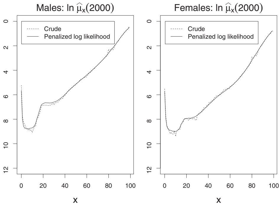
Figure 8 Observed and fitted forces of mortality for the year 2000: males and females
