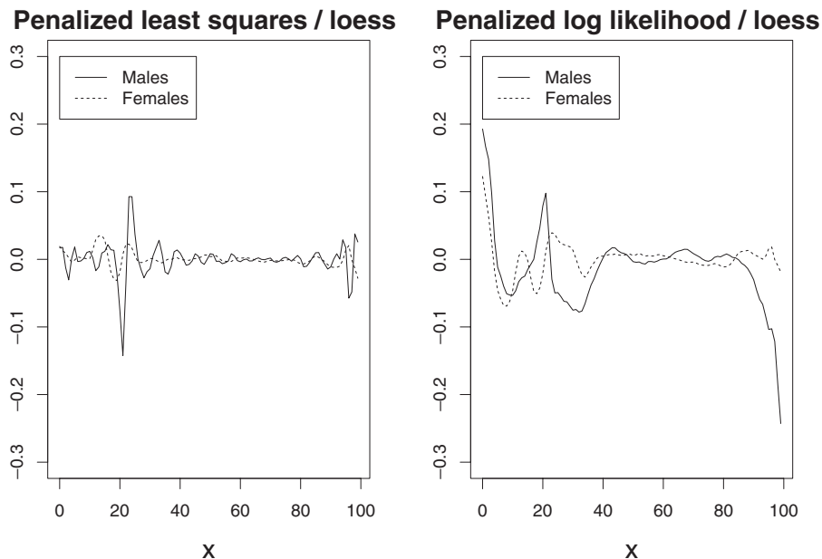
Figure 11 Relative differences of the smooth estimated \beta_x obtained from LOESS and penalized least squares (on the left) or penalized Poisson likelihood (on the right)
