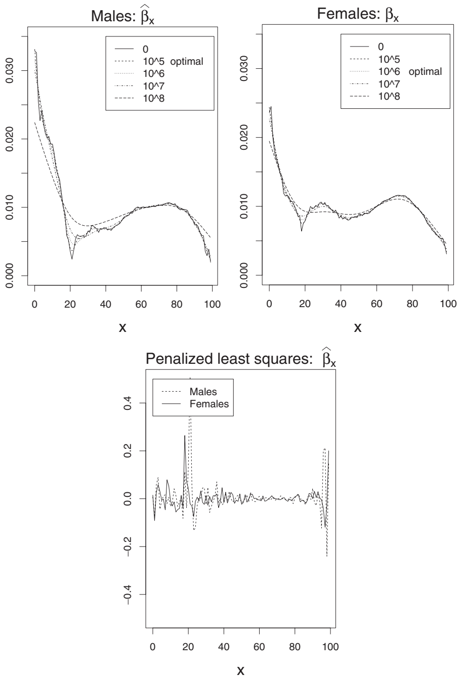
Figure 2 Estimation of the \beta_x parameters via penalized least squares for different values of \pi_\beta including the optimal \hat{\pi}_\beta selected by cross validation: estimated \beta_x 's for males (top left), estimated \beta_x 's for females (top right) and relative differences between the estimated \beta_x 's obtained without smoothing ( \pi_\beta = 0 ) and with the optimal smoothing coefficient \hat{\pi}_\beta (bottom)
