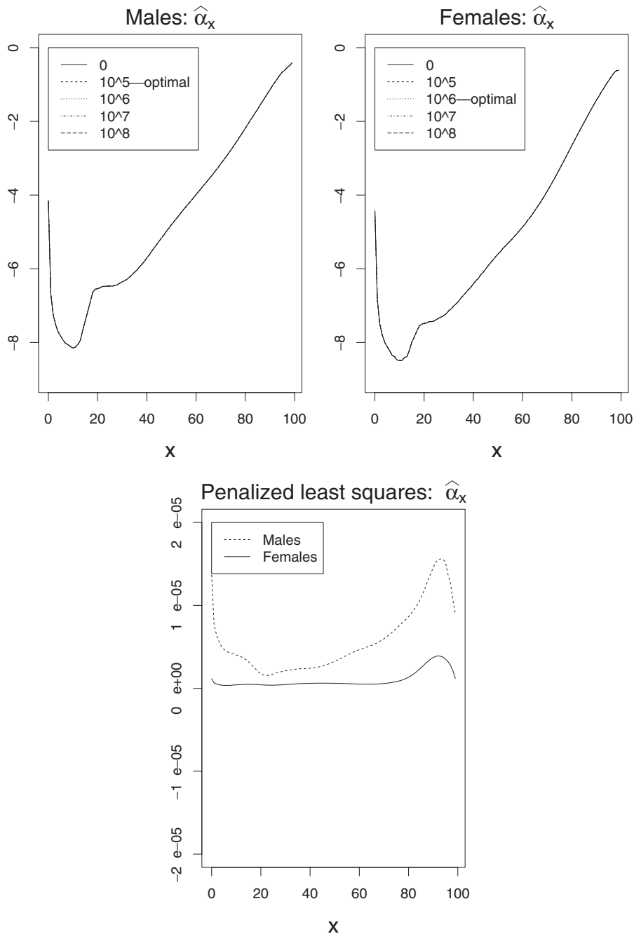
Figure 1 Estimation of the \alpha_x parameters via penalized least squares for different values of \pi_\beta including the optimal \hat{\pi}_\beta selected by cross validation: estimated \alpha_x 's for males (top left), estimated \alpha_x 's for females (top right) and relative differences between the estimated \alpha_x 's obtained without smoothing ( \pi_\beta = 0 ) and with the optimal smoothing coefficient \hat{\pi}_\beta (bottom)
