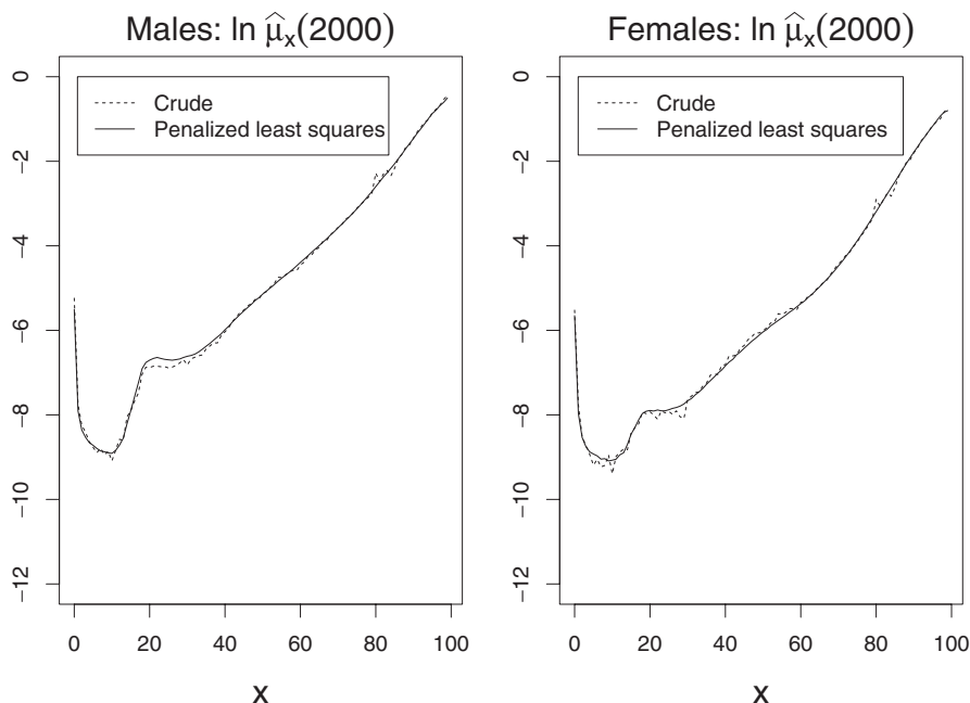
Figure 4 Observed and fitted forces of mortality for the year 2000: males and females
