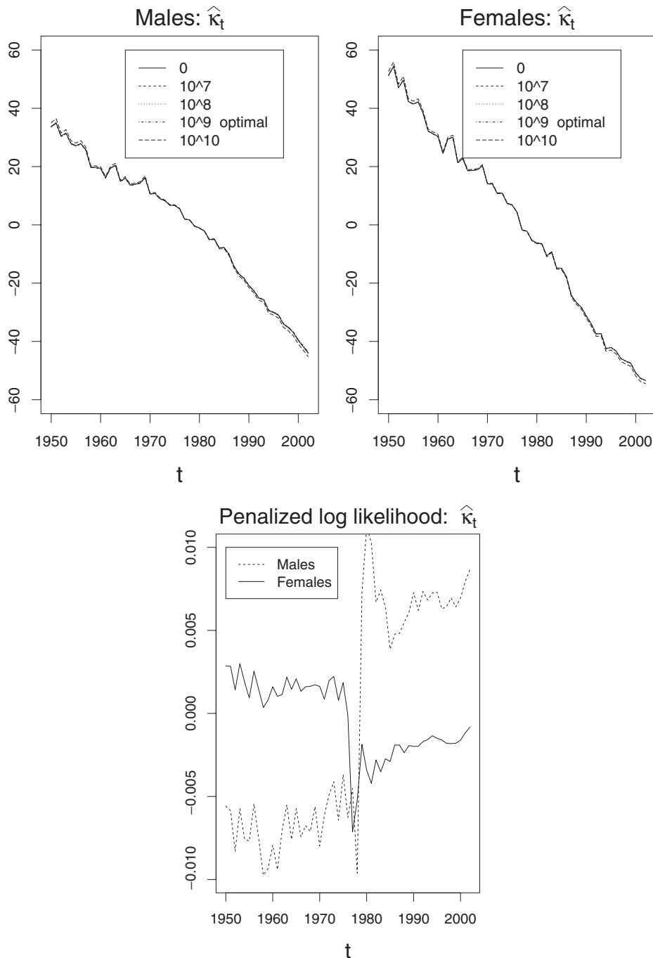
Figure 7 Estimation of the \kappa_t parameters via penalized maximum likelihood for different values of \pi_\beta including the optimal \hat{\pi}_\beta selected by cross validation: estimated \kappa_t 's for males (top left), estimated \kappa_t 's for females (top right) and relative differences between the estimated \kappa_t 's obtained without smoothing ( \pi_\beta = 0 ) and with the optimal smoothing coefficient \hat{\pi}_\beta (bottom)
