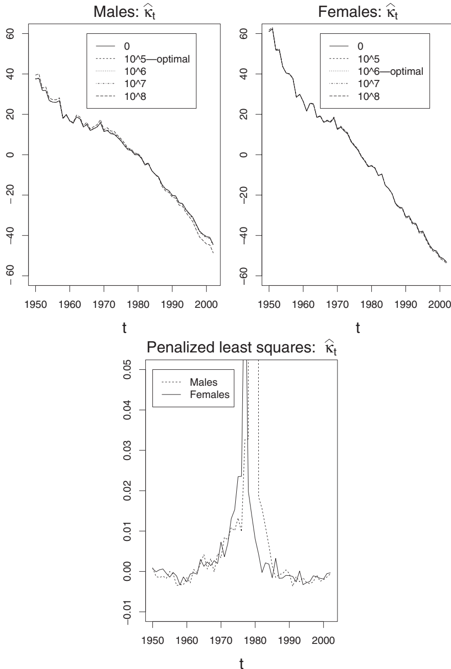
Figure 3 Estimation of the \kappa_t parameters via penalized least squares for different values of \pi_\beta including the optimal \hat{\pi}_\beta selected by cross validation: estimated \kappa_t 's for males (top left), estimated \kappa_t 's for females (top right) and relative differences between the estimated \kappa_t 's obtained without smoothing ( \pi_\beta = 0 ) and with the optimal smoothing coefficient \hat{\pi}_\beta (bottom)
