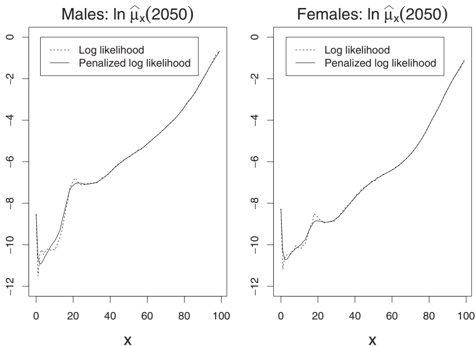
Figure 10 Forces of mortality for the French population in 2050 according to the smoothed Poisson log-bilinear model for mortality projection (males are on the left, females are on the right)
