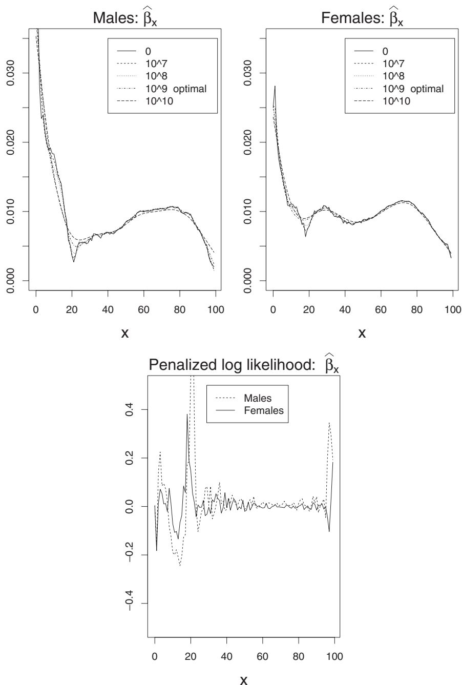
Figure 6 Estimation of the \beta_x parameters via penalized maximum likelihood for different values of \pi_\beta including the optimal \hat{\pi}_\beta selected by cross validation: estimated \beta_x 's for males (top left), estimated \beta_x 's for females (top right) and relative differences between the estimated \beta_x 's obtained without smoothing ( \pi_\beta = 0 ) and with the optimal smoothing coefficient \hat{\pi}_\beta (bottom)
